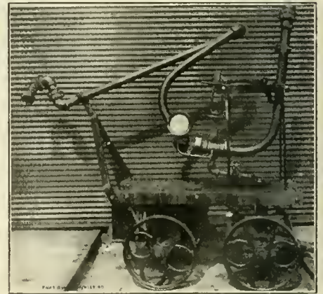
FIG. 3. TRUCK WITH PORTABLE CONNECTION FOR WATER CHANGING APPARATUS.
